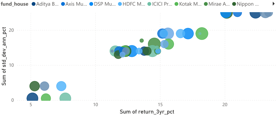
Risk vs Return Analysis
